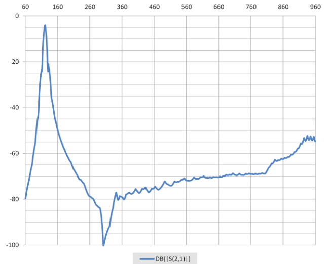
Out-Band Response (60 – 960 MHz)
