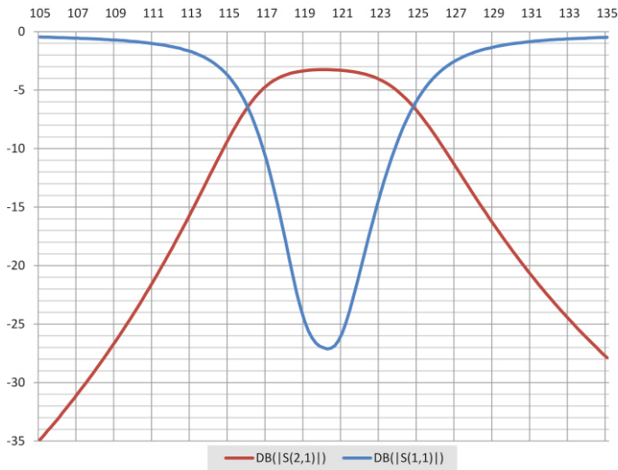
In-Band Response (105 – 135 MHz)
