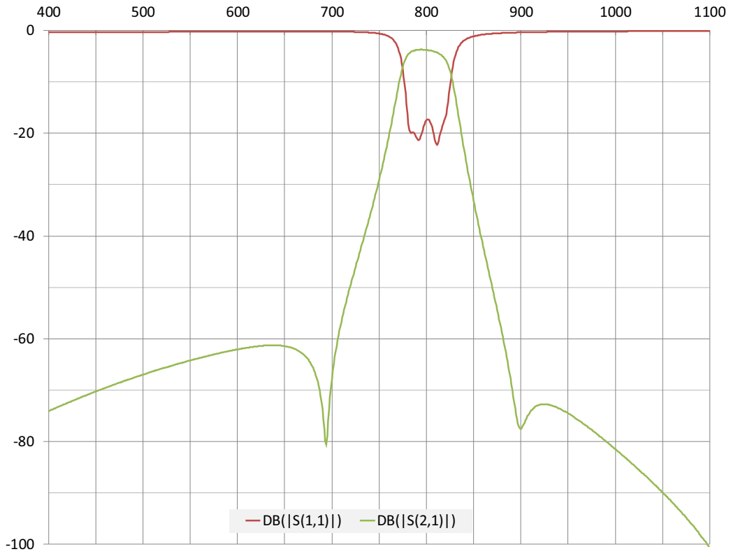
In-Band Response (400 – 1100 MHz)
